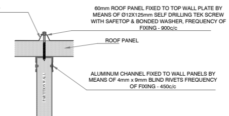
INTERNAL PARTITION WALL TO ROOF FIXING DETAIL
