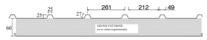
STD ROOF PANEL
