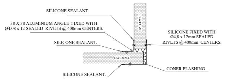
WALL TO WALL OUTSIDE CORNER FIXING DETAIL:
