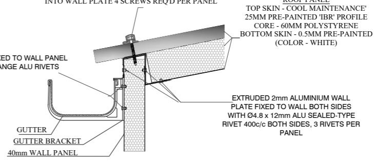
ROOF TO GUTTER DETAIL:
