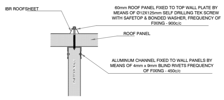
INTERNAL PARTITION WALL TO ROOF FIXING DETAIL
