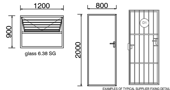
EXAMPLES OF TYPICAL SUPPLIER FIXING DETAILS
