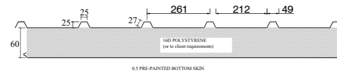
STD ROOF PANEL
