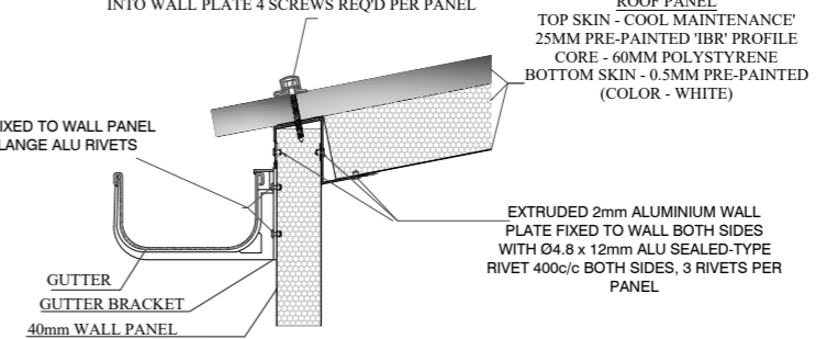
ROOF TO GUTTER DETAIL:
