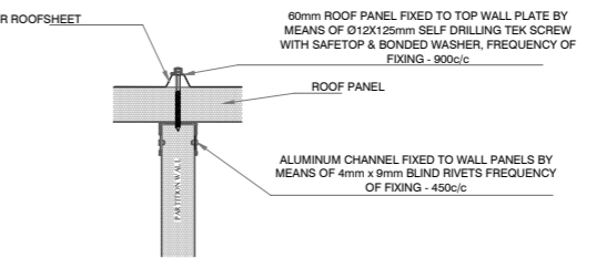
INTERNAL PARTITION WALL TO ROOF FIXING DETAIL
